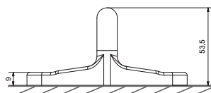
Ground configuration
