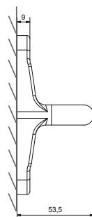
Wall configuration
