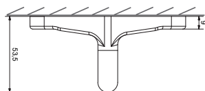
Ceiling configuration
